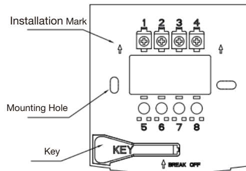
Figure 2: K600 Callpoint Base
