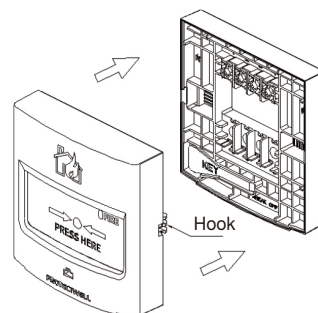
Figure 4: Mounting
